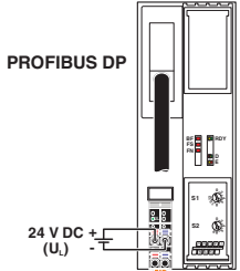
Connection diagram
